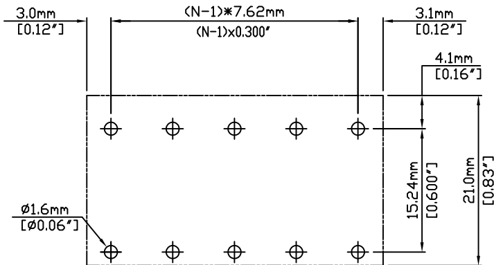
PCB. LAYOUT
